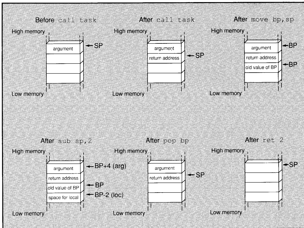
Figure 17.2 Local Variables on the Stack
