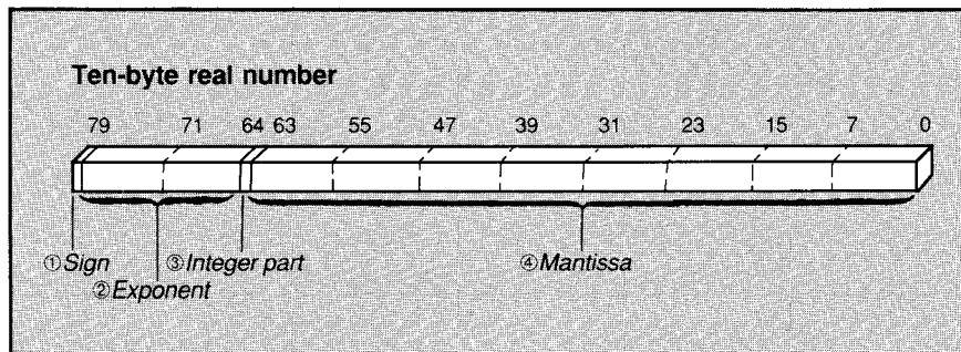
Figure 6.3 Encoding for Real Numbers in Temporary-Real Format
