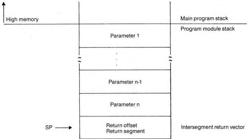
Figure 10.1 Contents of Stack at Entry to a Routine
