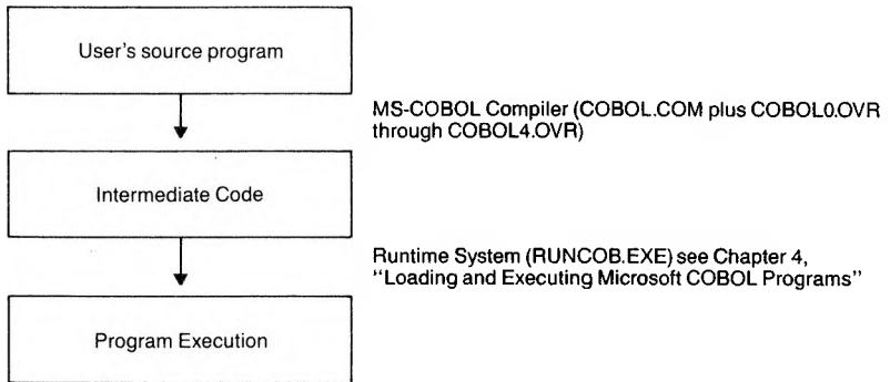
Figure 2.1 Major Steps in Compiling and Executing an MS-COBOL Program
