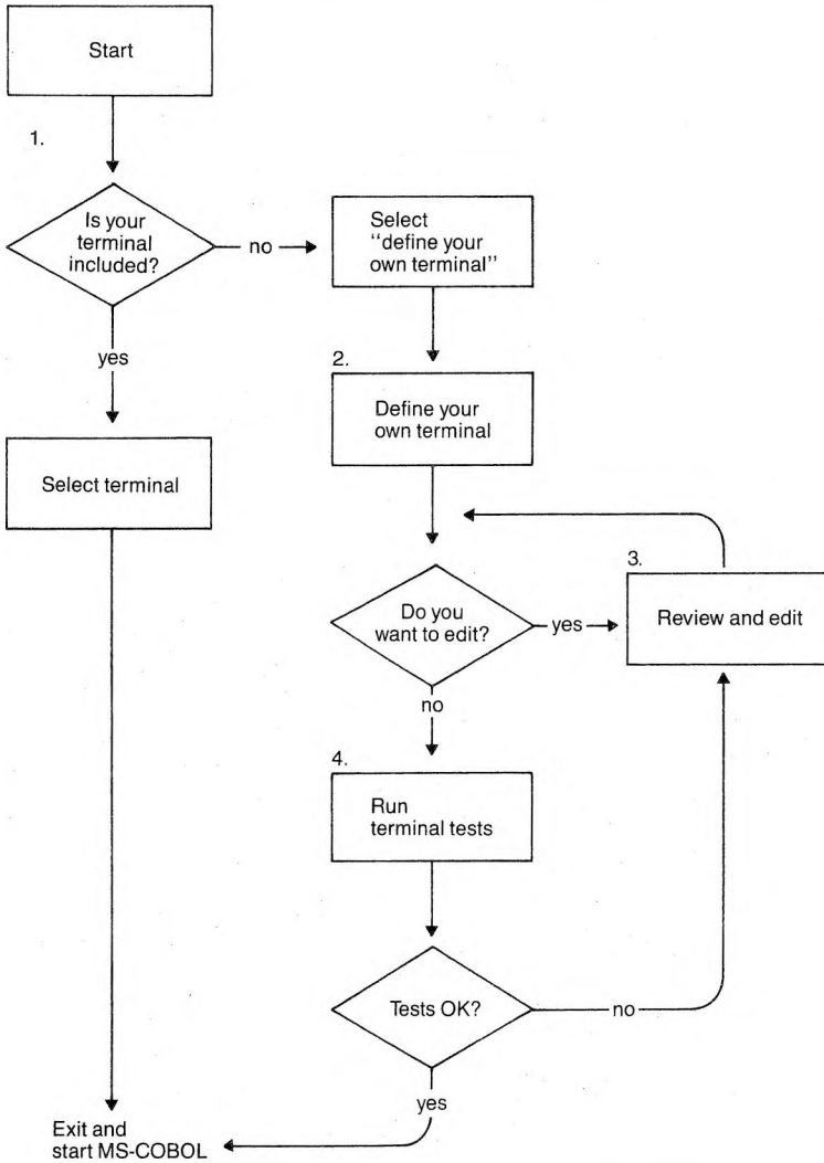
Figure 9.1 INSTALL Program Steps
