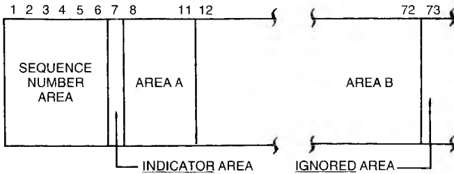
Figure 2.1. Format of MS-COBOL Source Line
